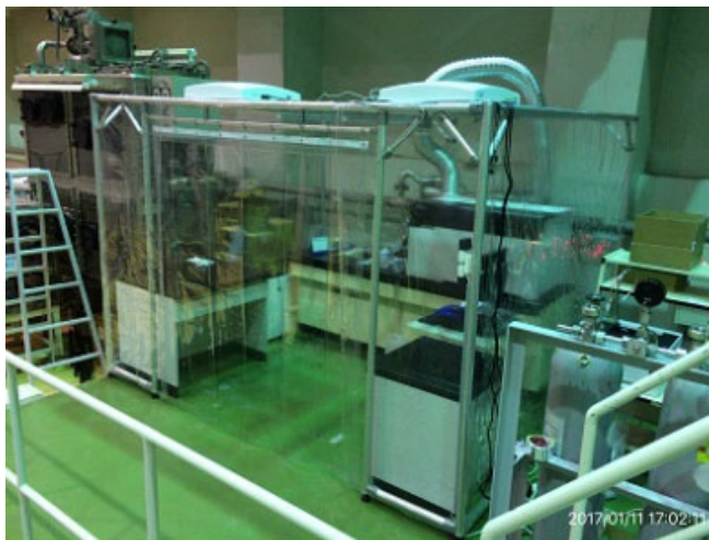
ICP-MS/MS, Agilent 8900
